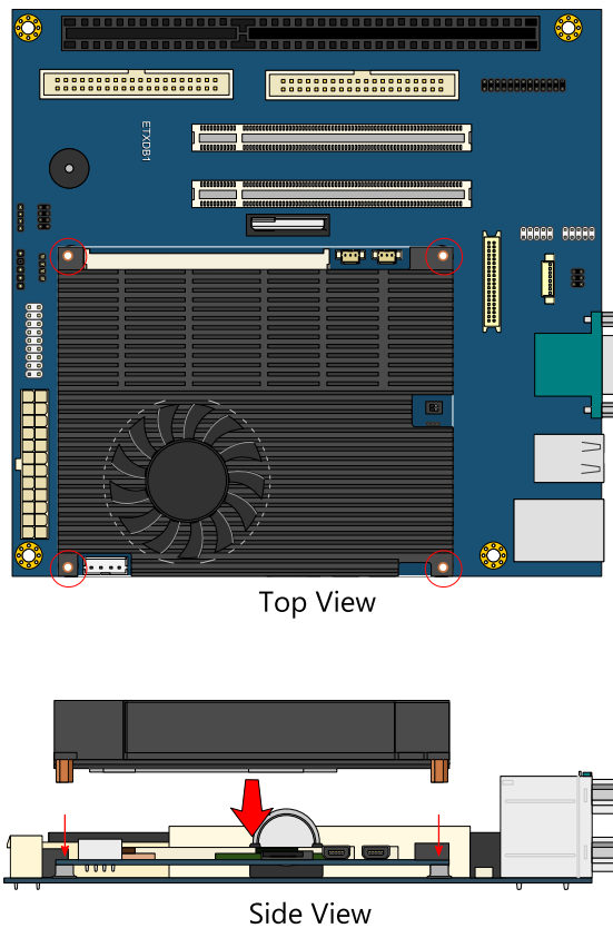
Figure 21: Installing the heatsink/heat spreader on VIA ETX-8X90 module
