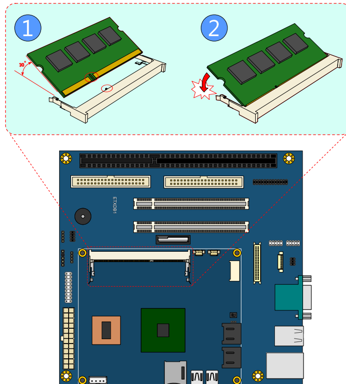
Figure 18: Installing the DDR3 SODIMM memory module
