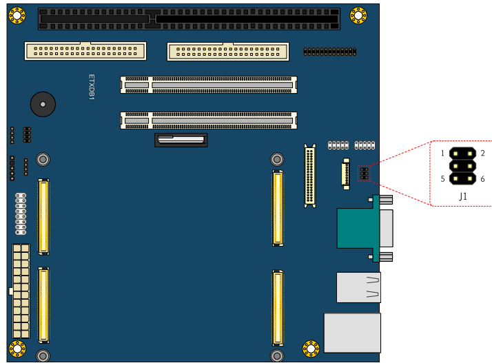
Figure 54: Backlight and Panel power jumper diagram
